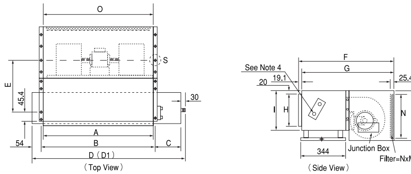
Figure 3 : HCCA Unit With Bottom Return Plenum
