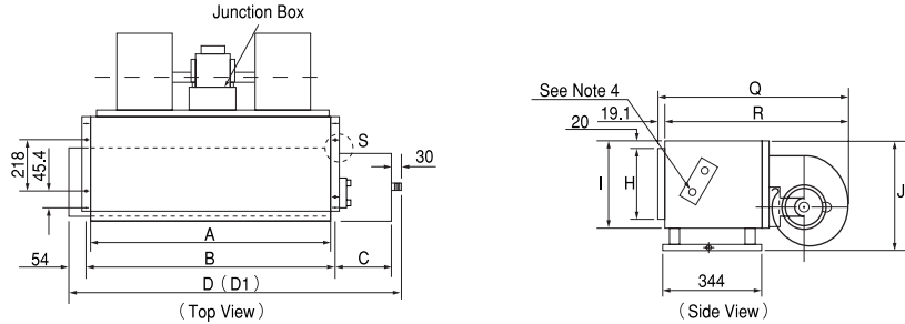
Figure 2 : HCCA Unit With Rear Return Plenum
